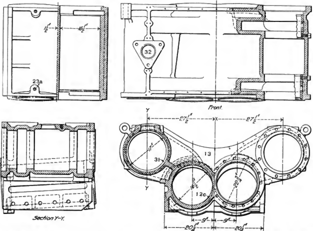
Figs. 836-839. High Pressure Cylinders of Cole Four-Cylinder Balanced Compound Locomotive, Diameter 16½ in. American Locomotive Co.
